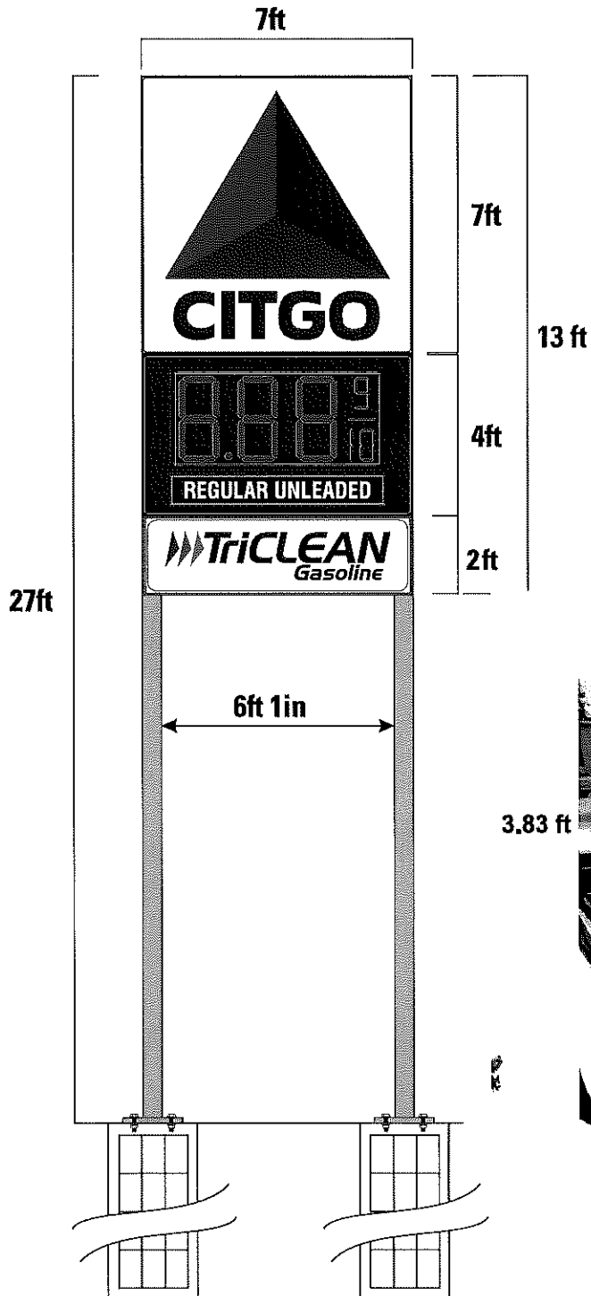
ELEVATION DETAIL
